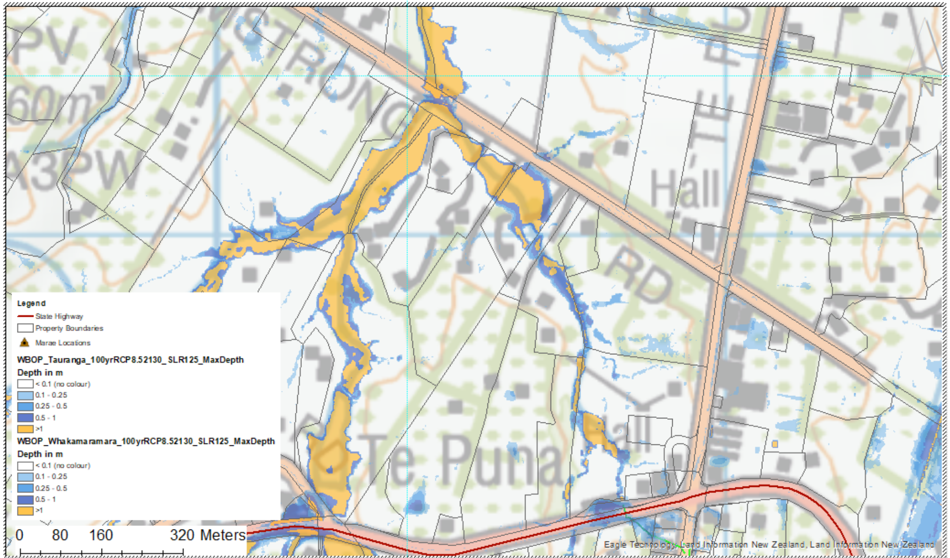
Figure 4: existing flood depth downstream – zoomed in
