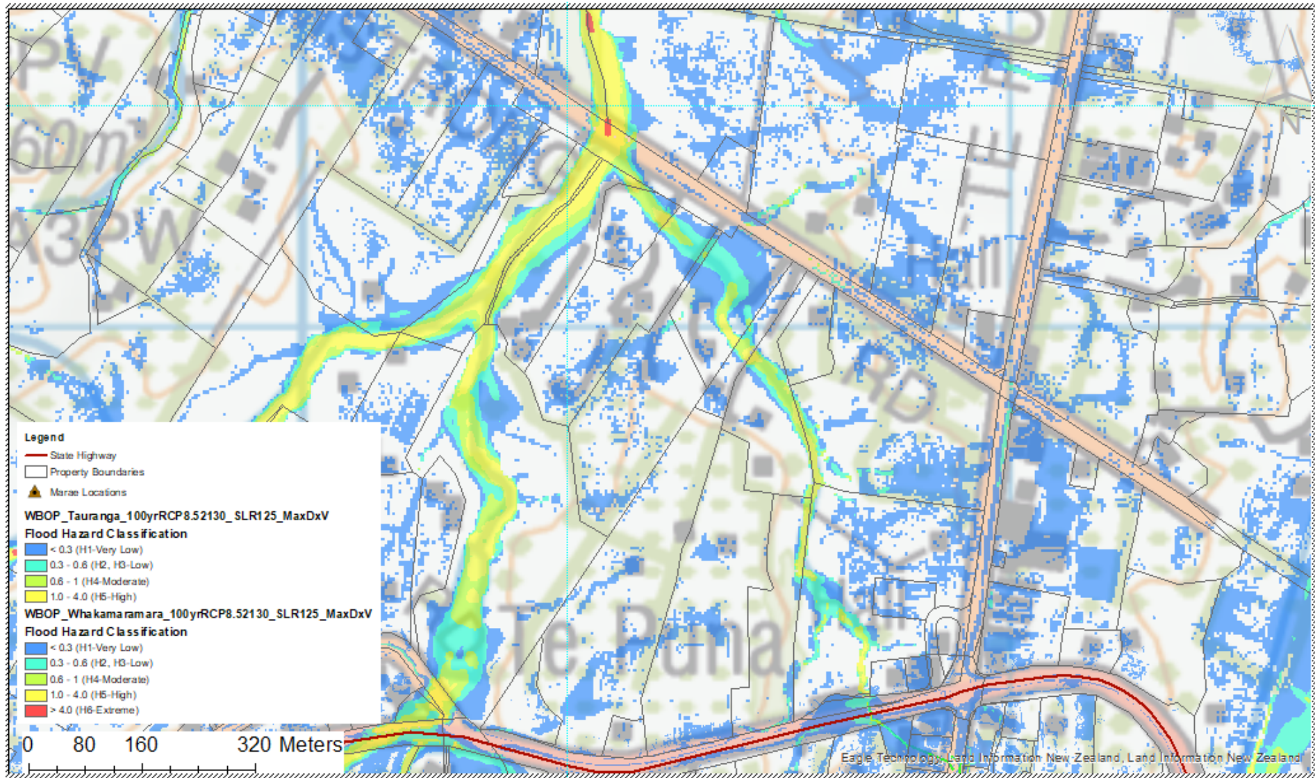
Figure 9: existing max DxV downstream – zoomed in
