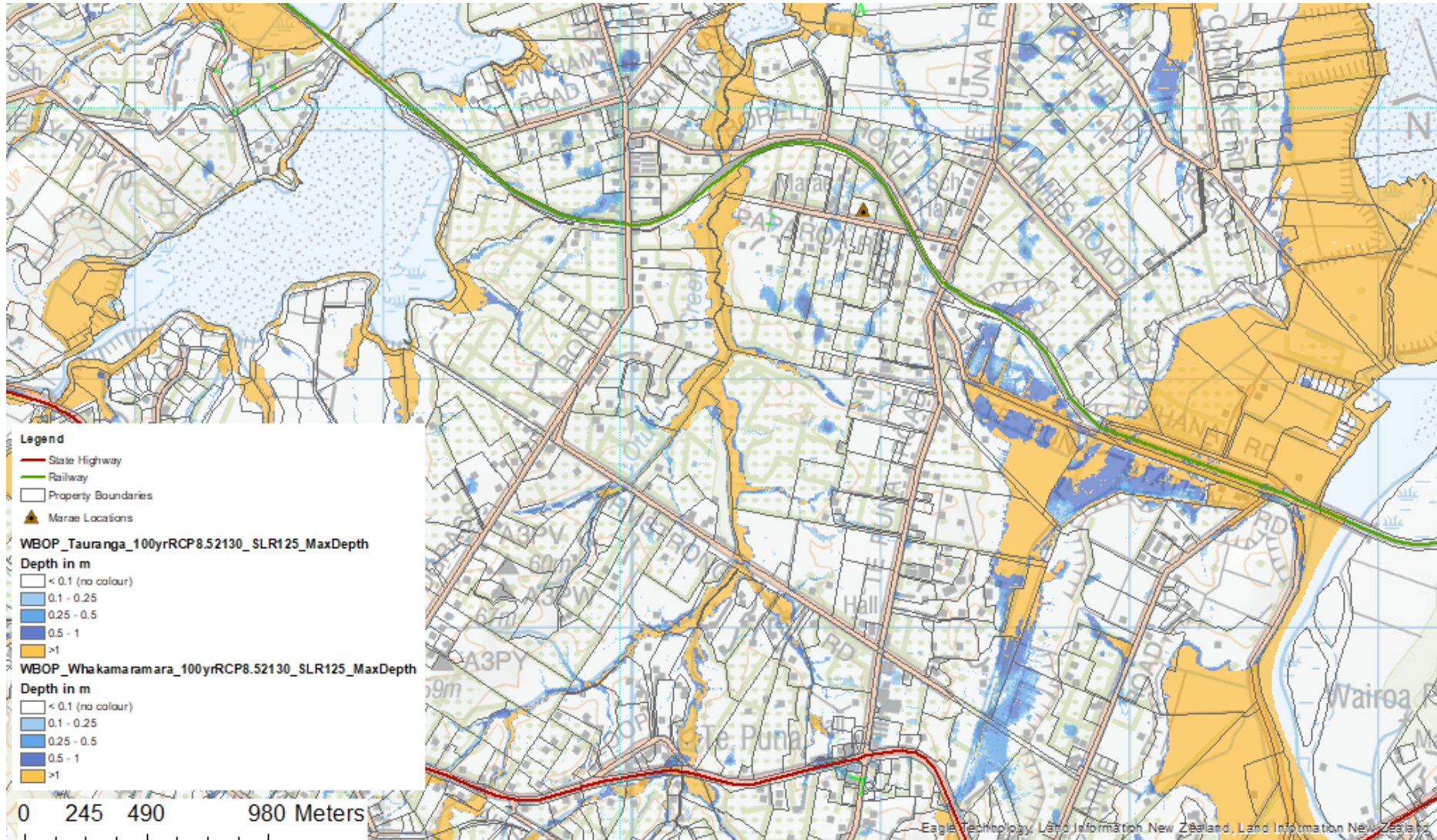
Figure 3: existing flood depth downstream
