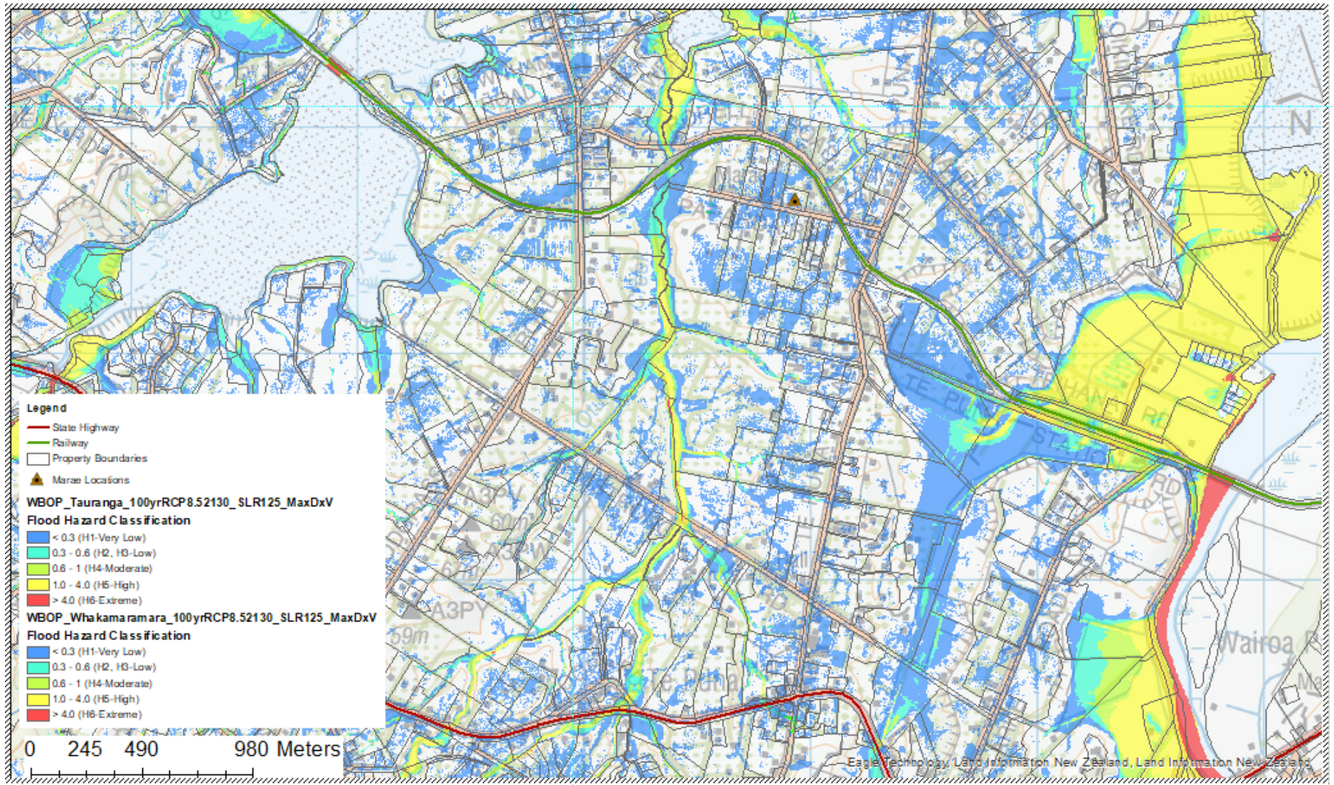
Figure 8: existing max DxV downstream
