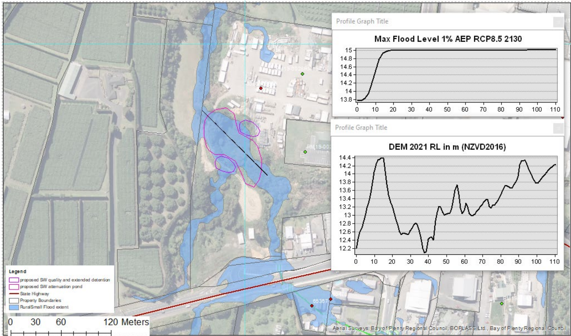
Figure 7: existing flood extent on site and dam impact on flood levels
