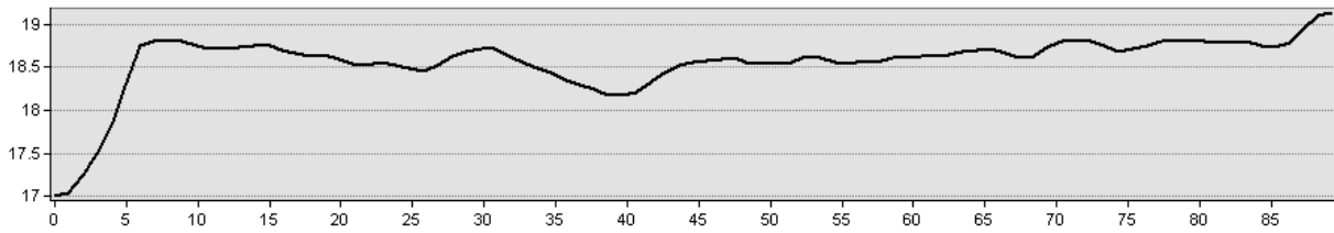
Post-development levels – long section through pond
