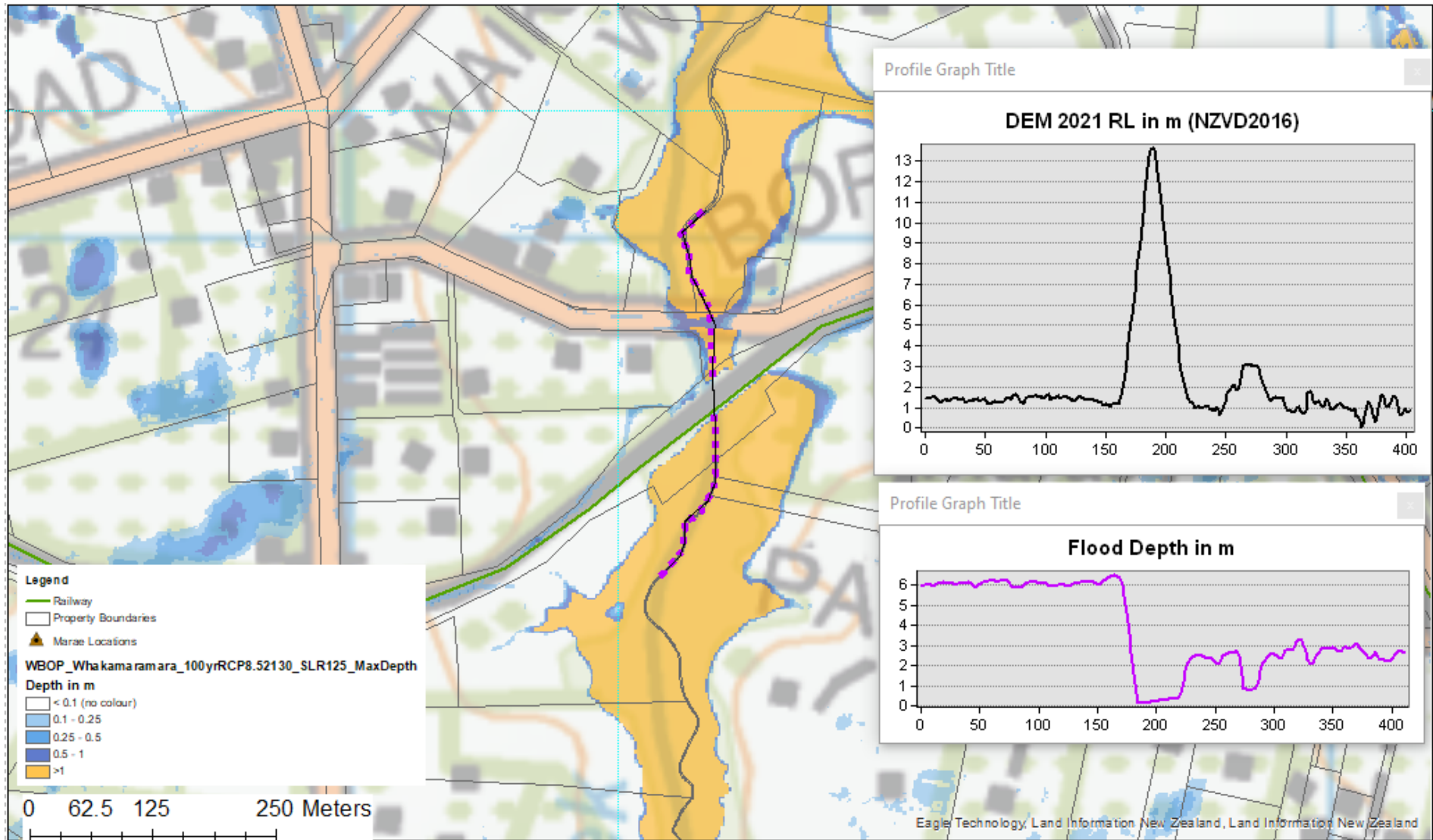
Figure 5: existing flood depth downstream – Borell Road & Railway zoomed in
