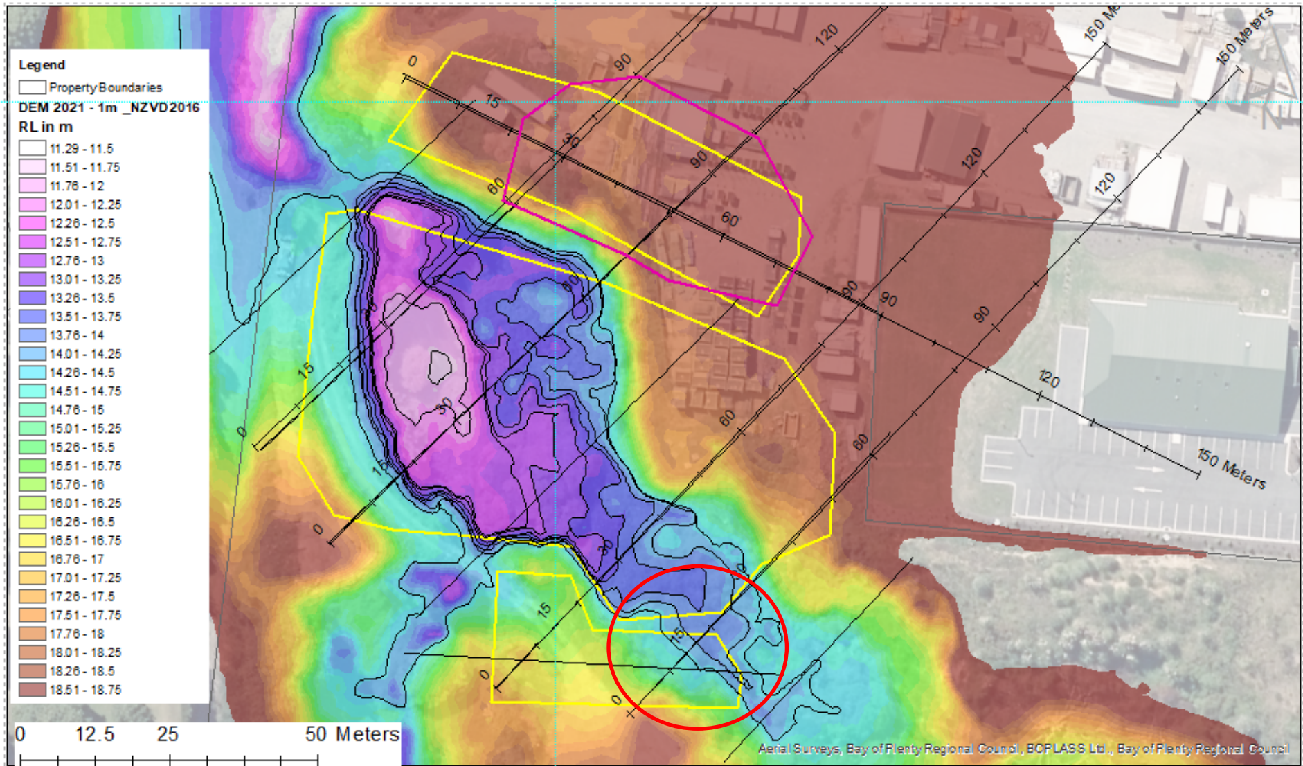
Figure 12: investigation southern constructed treatment and extended detention wetland
