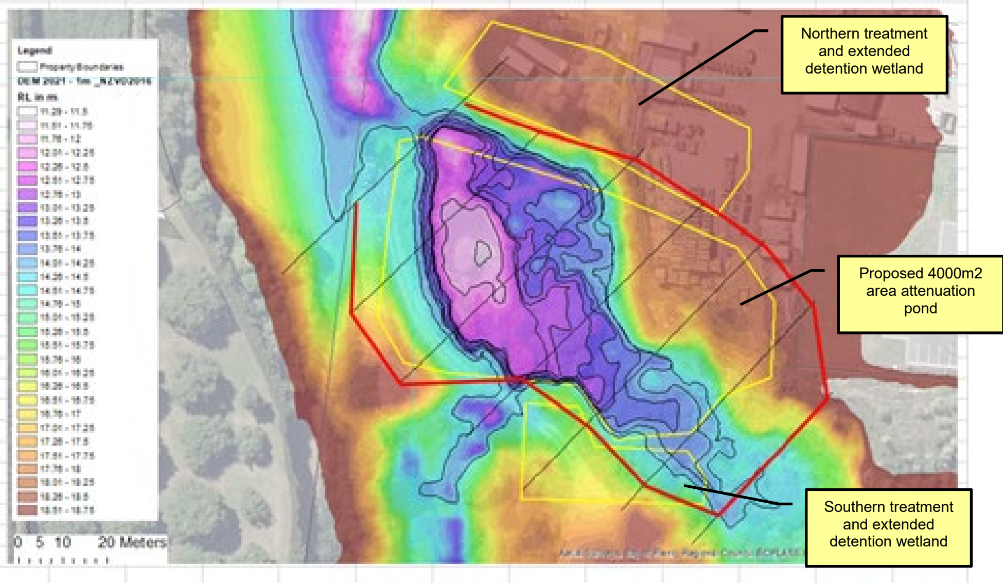
Figure 10: investigation on-line attenuation pond
