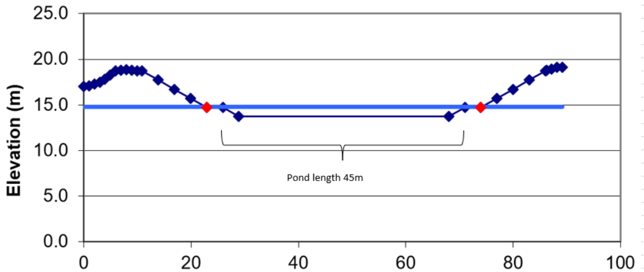
Figure 11: investigation northern constructed treatment and extended detention wetland
