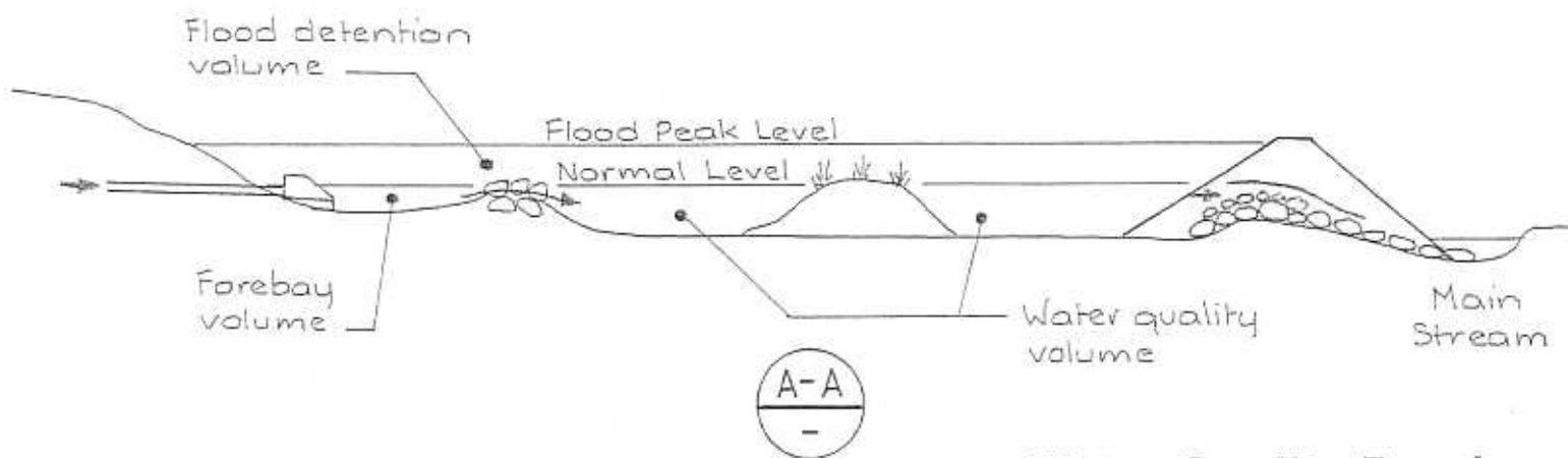
Water Quality Ponds, Forebays & Flood Detention Ponds
